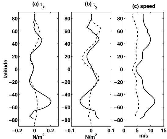
Figure 5: Annual average (a) zonal wind stress ( N m^{-2} ); (b) meridional wind stress ( N m^{-2} ); (c) wind speed ( m/s ). Solid line is from Trenberth et al. (1989); dashed line is from atmospheric model.
