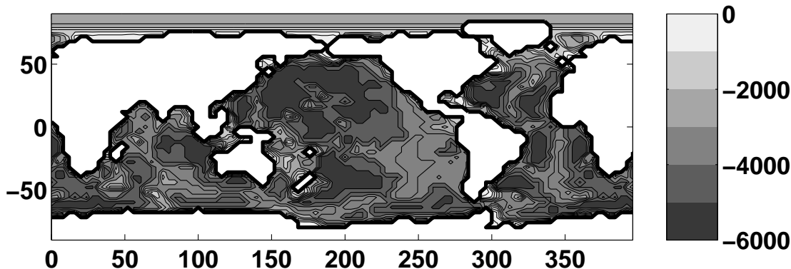
Figure 2: Ocean model bathymetry (m) used in the example simulation discussed in Section 4. Contour interval is 500m.
