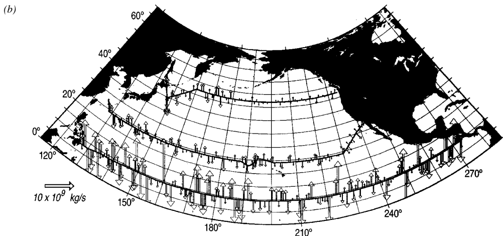
Figure 1 (a) A section (after Dietrich et al 1975) showing the large-scale patterns of oxygen concentration in a section running meridionally through the Pacific Ocean. These patterns have traditionally been interpreted to imply the dominance of a simple, large-scale, nearly unchanging flow field. (b) Instantaneous mass transports in the depth range roughly between 200 and 1000 m perpendicular to the three ship tracks, as estimated by Macdonald (1995). The very large spatial variability (and an implied temporal variability) undermines the idea that a simple laminar flow field produces the large-scale oceanic property distributions. (c) Hodograph plot (meridional component of velocity, v , as a function of the zonal component, u ) from two years of daily average velocities from a current-meter record at 41^\circ\text{N} , 175^\circ\text{W} , 135-m depth, in the North Pacific Ocean. The lack of temporal stability is evident.
