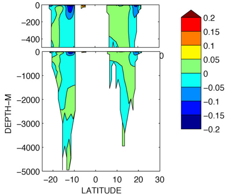
Fig. 6. 15-Year average zonal flow in Section 2B, U_{2B} , at 114.5^\circ\text{E} (m/s). No obvious simple reference level for thermal wind calculations emerges.
