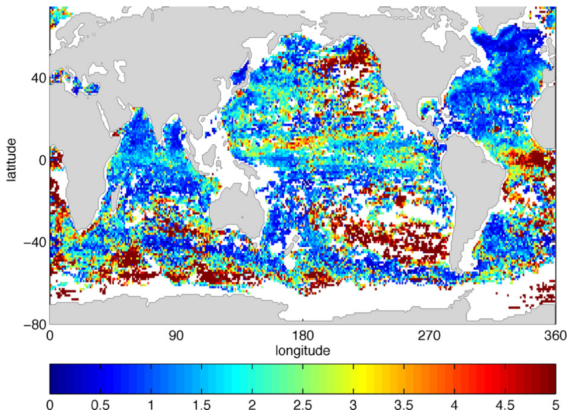
Fig. 1. The vertical and time average (not depth-weighted) misfit to 16 years of profiling float temperature data, although most of the observations (Argo) are confined to the interval since 2001. In an ideal solution, in which the expected errors were also known perfectly, the misfits would be spatial white noise obeying a \chi^2_1 distribution. Some spatially systematic misfits are observed, e.g., in the southeast Pacific Ocean, although whether they represent model difficulties, data calibration issues, or simply a still unconverged solution, is obscure. The misfits are dominated by the very deepest values near 2000 m. Indian Ocean salinity misfits (not shown) are believed to arise primarily from calibration errors in the data. Misfits are, by definition, dimensionless.
