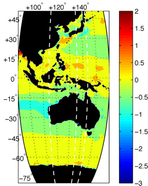
Fig. 22. Time-mean net fresh water flux (positive into the ocean) 10^4 \text{ kg/m}^2/\text{s} . The region is one of intricate spatial variation in the precipitation minus evaporation pattern but is one of net precipitation in the regions north and east of the ITF.
