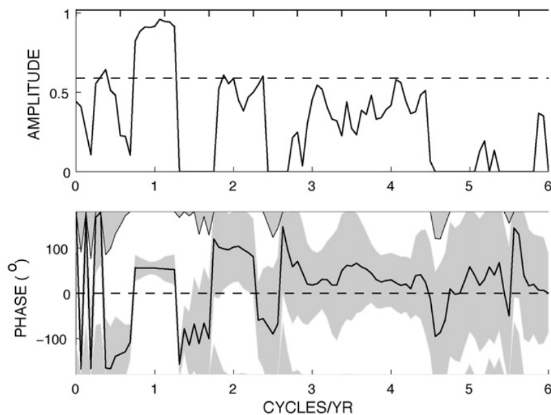
Fig. 15. Coherence of the pressure difference \eta_{EAST} - \eta_{WEST} with the total transport through Section 2B. Strong coherence exists in the annual band, but whatever exists at lower frequencies below the level of no significance and would at most, account for 15% of the variance in that band. Gray band is the estimated 95% confidence interval for the coherence phase.
