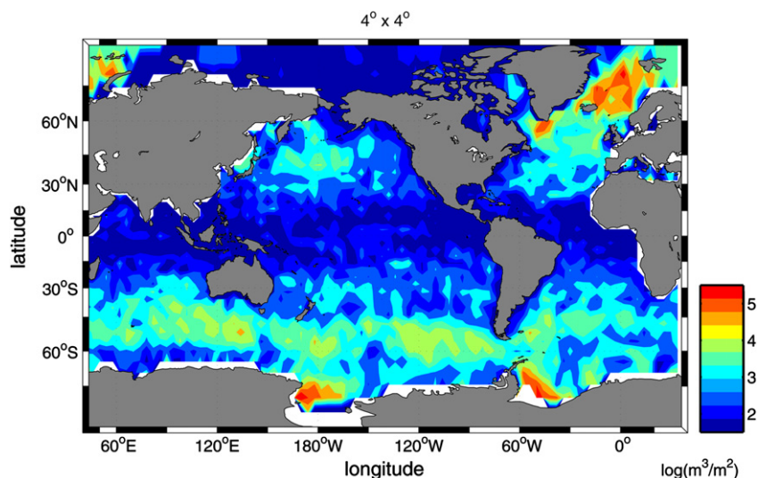
Fig. 4. Ocean volume whose last contact with the surface occurred in each 4 × 4° square in m 3 of volume/m 2 of surface area. A logarithmic scale is used (Gebbie and Huybers, (2010), who show a higher resolution version of this plot). Courtesy of G. Gebbie.
