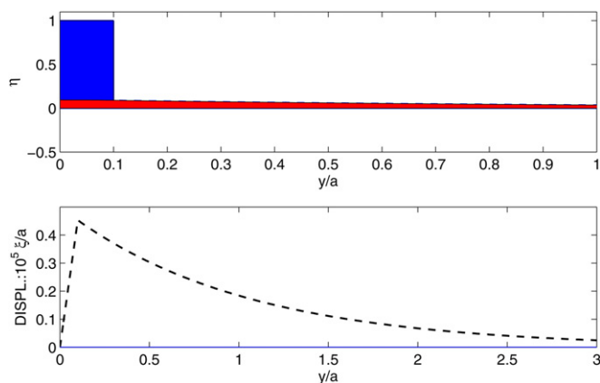
Fig. 5. Upper panel. Initial surface elevation or bottom pressure anomaly (blue) for the special case y_1 = a/10 , and after geostrophic adjustment. a is the barotropic deformation radius. Lower Panel. Non-dimensional lateral displacement of the fluid after adjustment, but which is a very small fraction of the distance disturbed, so that the fresh water distribution is little changed from its initial position, although it is assumed to have achieved local isostatic equilibrium. Note the differing horizontal scales. (Wunsch, 2010, unpublished ms.).
