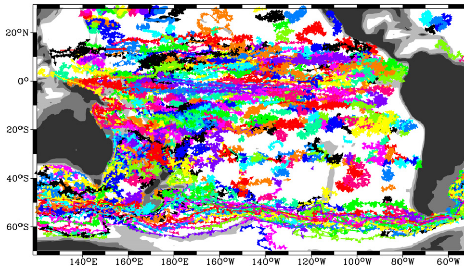
Fig. 1. From Davis (2005) showing trajectories of neutrally buoyant floats deployed in the Pacific Ocean (mainly) at a nominal depth of 900m. The result shows little evidence of the large-scale meridional flows of the Stommel-Arons theory, nor does it suggest much in the way of a “conveyor belt” circulation. (Courtesy of R. Davis, 2010).
