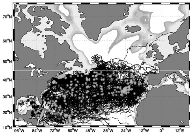
Fig. 3. From Brambilla and Talley (2006) showing trajectories of surface drifters launched south of 45°N. With one exception, none of them enters the sub-polar gyre. The nominal depth measured is 15m. Drifters were launched between 1990 and 2002 (Courtesy E. Brambilla).
