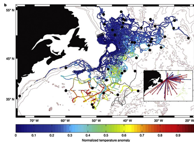
Fig. 2. Two-year trajectories of floats released in the so-called Labrador Sea Water at 700 and 1500m depths. Of the 55 available float tracks, only 4 entered the Deep Western Boundary Current in the sub-tropical gyre (updated from Bower et al., 2009). But how much more interesting and useful it is to ask whether these data are not telling a completely different story! (Courtesy, A. S. Bower, 2010).
