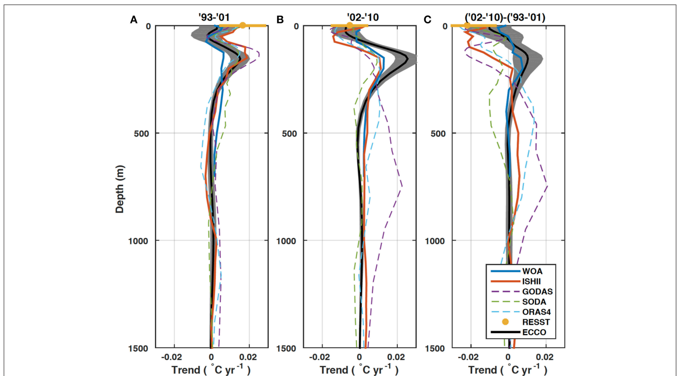
FIGURE 1 | Decadal trends in global mean potential temperature as function of depth over the periods 1993–2001 (A), 2002–2010 (B), and their difference (C), inferred from two hydrographies, three ocean reanalysis and the ECCOV4 state estimate. Black: ECCOV4 (gray shading indicates formal standard error, see main text), dark blue: WOA (Levitus et al., 2012); red: Ishii (Ishii et al., 2005); purple: GODAS (Huang et al., 2010); green: SODA (Carton and Santorelli, 2008); light blue: ORAS4 (Balmaseda et al., 2012); yellow: SST (Reynolds et al., 2002). Adapted from National Academies of Sciences, Engineering, and Medicine (2016) (their Figures 4, 23).
