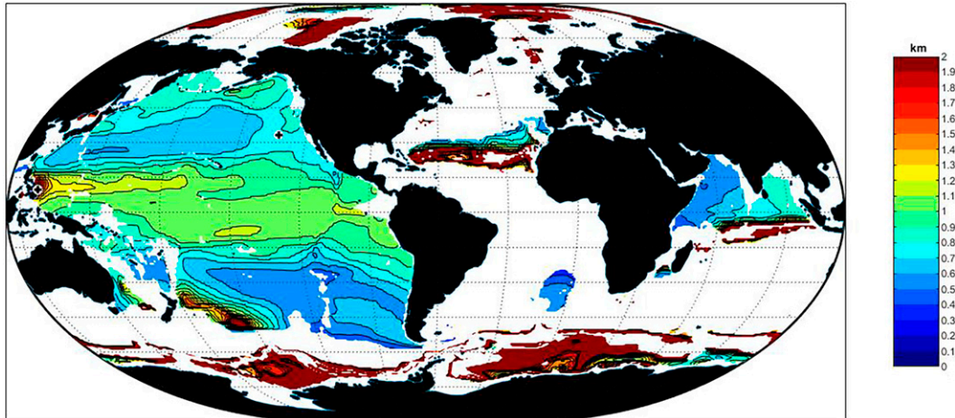
FIG. 13. Significant values of the salinity scale height (km). Color saturates at 2 km.
