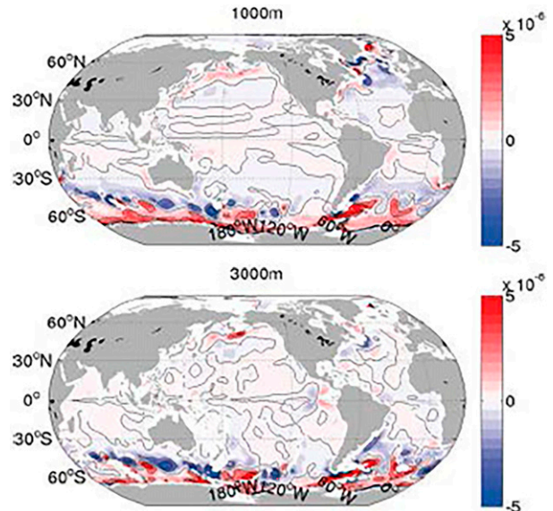
FIG. 3. Time-mean vertical velocity w ( \text{m s}^{-1} ) at two depths, from an ECCO state estimate ( Liang et al. 2017 ). The relatively small scales appearing in the Southern Ocean and high northern latitudes are notable, along with the much larger-scale features at midlatitudes, particularly the zonality visible at 1000 m.
