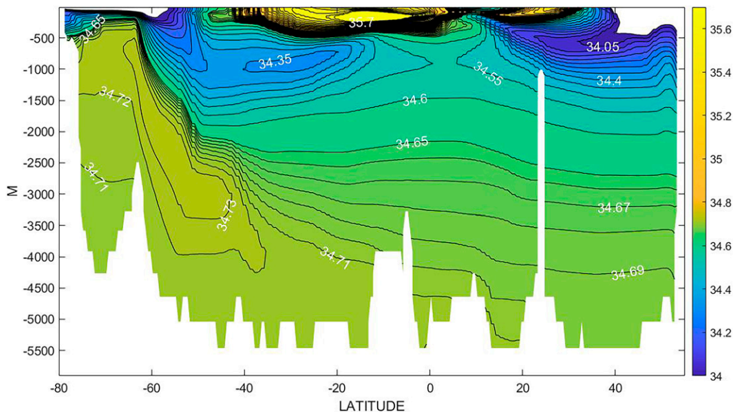
FIG. 2. 26-yr time-average salinity field along meridian 165^{\circ}\text{W} from ECCO results. Compare to WOCE line P15. Here, and in other figures, colors saturate at the extremes.
